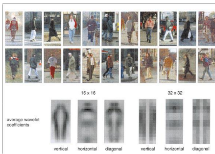
SVM with Haar wavelets [Papageorgiou & Poggio, IJCV 2000]
